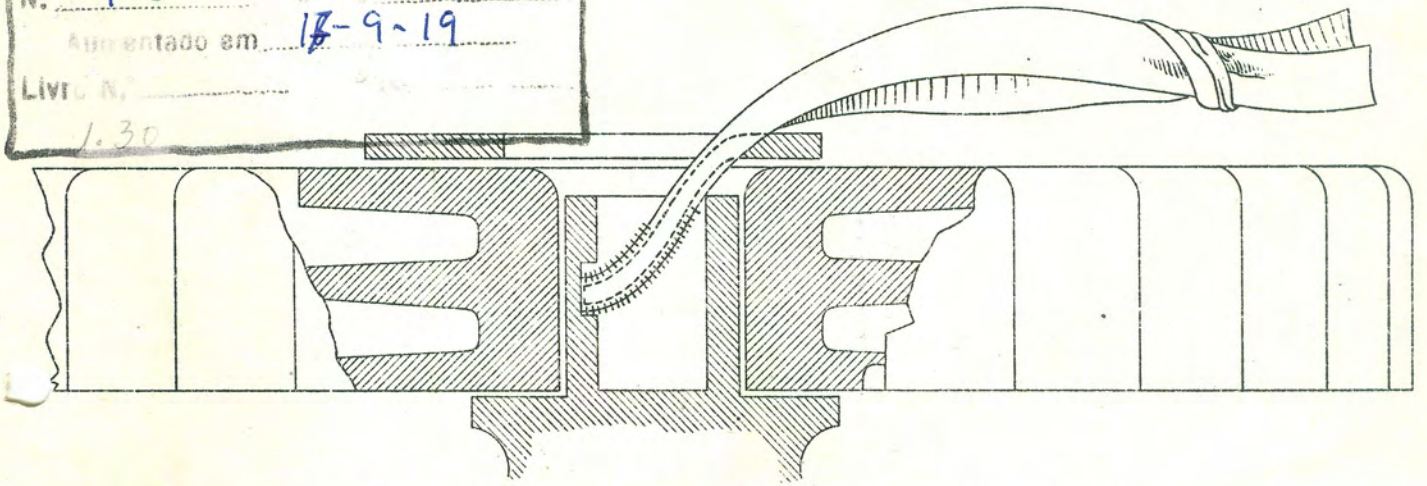
SECTION THROUGH MAGAZINE.
